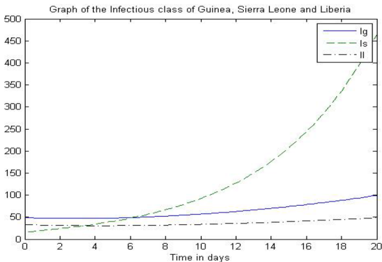
Figure 1: The graph of infectious class of Guinea, Sierra Leone and Liberia, using the data of 2014.
