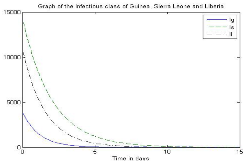
Figure 2: The graph of infectious class of Guinea, Sierra Leone and Liberia, using the 2016 data.
