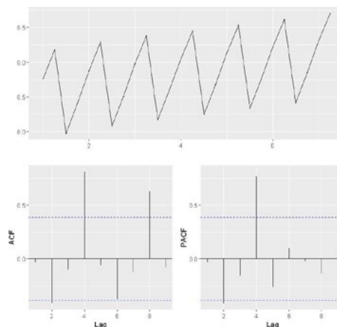
Figure 9: Peasant per capita disposable income time series model residuals ACF and PACF.
