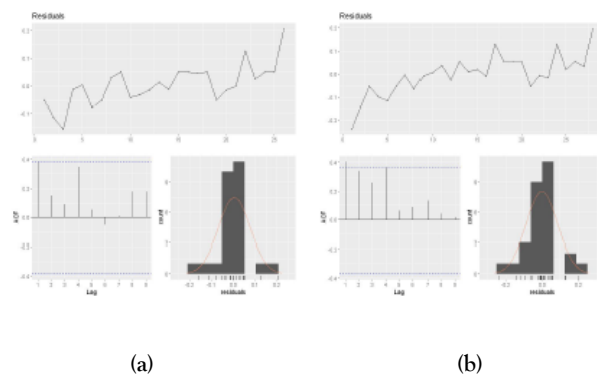
Figure 7: Model comparison with forecast residual graph; (a) Model comparison residuals; (b) The model predicts residuals.
