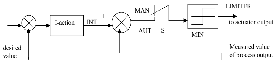
Figure 1: Practical realisation of integral regulator.
